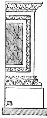
Fig. 527. Pedestal of Trajan's Column.
